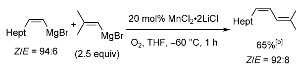
Scheme 5. Preparation of conjugated dienes by Mn-catalyzed oxidative heterocoupling. [a] [a] For the stereoselective preparation of ( Z )-1-nonenylmagnesium bromide, see Supporting Information. [b] For selectivity, see Table S1 in the Supporting Information.
