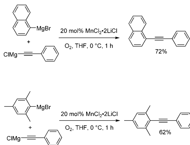
Scheme 2. Oxidative heterocoupling of aryl- and alkynyl Grignard reagents.
